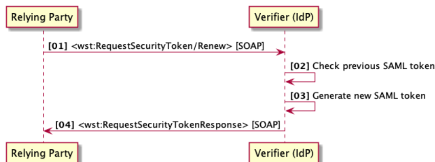
Figure 3: Renewal of a SAML-Assertion
