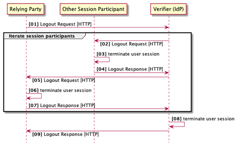
Figure 6: OpenID Connect Logout Sequence
