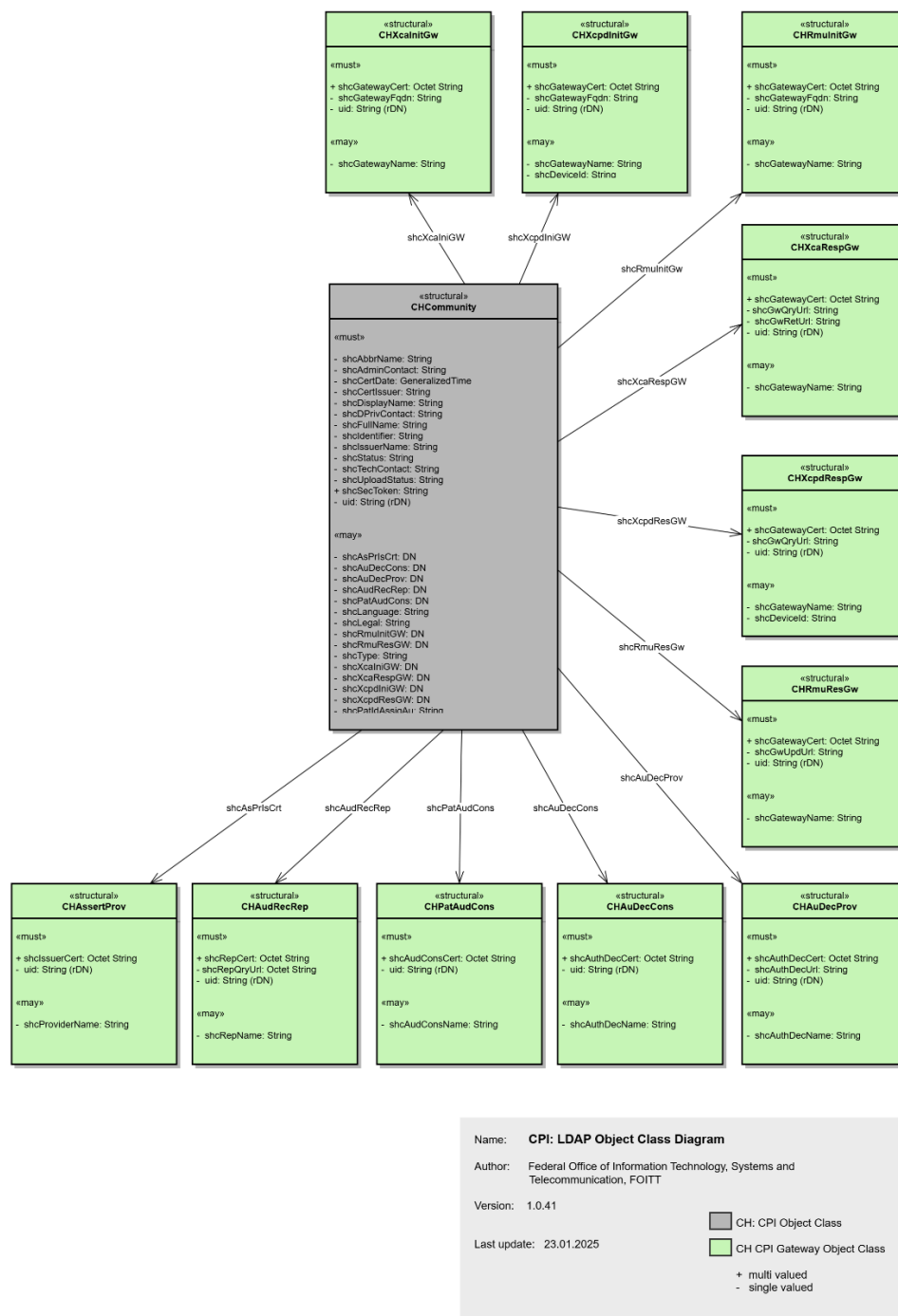
Figure 13: CH:CPI LDAP Schema
