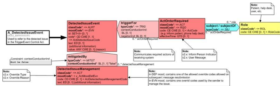
Figure 7: RIMM for DetectedIssueEvent
